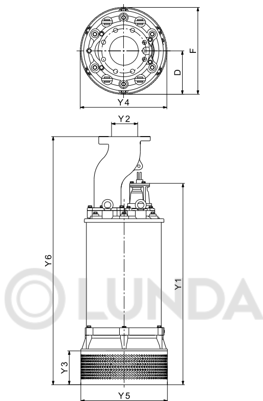
Fig. 4 Dimensions of pump with flange connection
