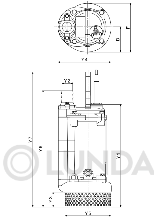
Fig. 1 Dimensions of pump with hose connection
