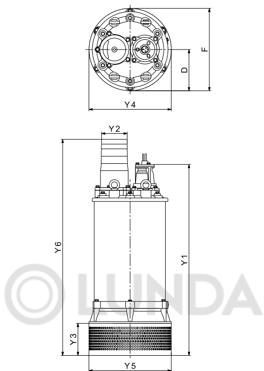
Fig. 3 Dimensions of pump with hose connection
